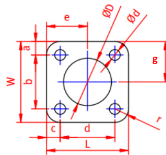
FOUR BOLT FLANGE
