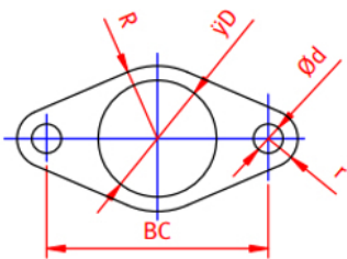
TWO BOLT FLANGE
