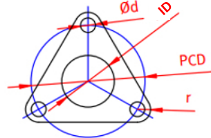
THREE BOLT FLANGE
